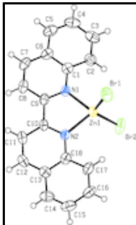
Fig. 1. The molecular structure of the title molecule, with the atom-numbering scheme. Displacement ellipsoids are drawn at the 50% probability level.
