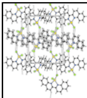
Fig. 2. Packing diagram for title molecule viewed down the a axis. Dashed lines indicate weak C—H...Br intermolecular interactions.
